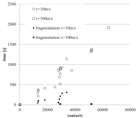
Fig. 16. Total computation time and computational time of fragmentation per number of contacts at each simulation step for crushing velocities of v = 10 m/s and v = 100 m/s.
