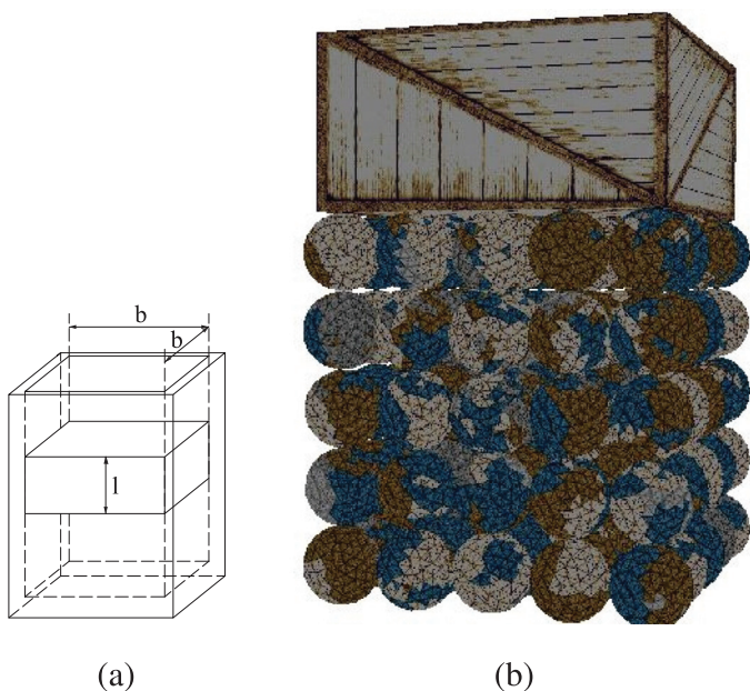
Fig. 13. Geometry of container and fragment pattern. (a) The dimension of the container is b \times b , where b = 6\text{ cm} . The depth of the hammer is l = 25\text{ m} . (b) Fragment distribution after impact for DCF2 colored by particle.
