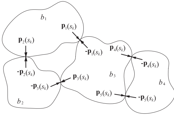
Fig. 3. Collision of multiple bodies: multiple bodies, \mathbf{b} = \{b_0, b_1, \dots, b_m\} , collide with multiple contact points \mathbf{c} = \{c_0, c_1, \dots, c_n\} , m is the total number of colliding bodies and n is the total number of contact points. A set of impulses, (\mathbf{p}_0(s_k), \mathbf{p}_1(s_k), \dots, \mathbf{p}_n(s_k)) , are applied to contact points at iteration s_k .
