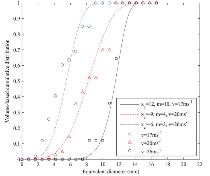
Fig. 11. Cumulative volumetric size distribution of fragments from fragmentation process depicted in Fig. 10.
