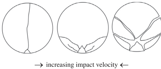
Fig. 2. Fragmentation modalities at increasing impact velocities (adapted from Salman et al., 2004 ).
