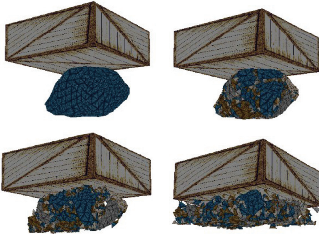
Fig. 10. Progressive fragmentation sequence for crushing of an irregularly-shaped rock block, with an initial crushing velocity of 26 m/s.
