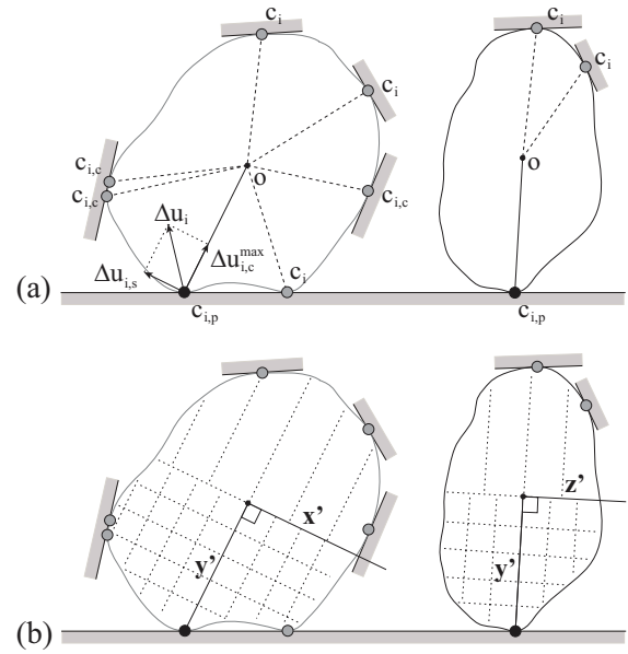
Fig. 4. Contact distribution and seed placement. (a) Local coordinate system at the primary contact, c_{i,p} . \mathbf{o} is the geometry center of the colliding body. \mathbf{y}' is the primary axis of fragmentation, \mathbf{x}' is the secondary axis, and \mathbf{z}' is orthogonal to both \mathbf{x}' and \mathbf{y}' . \Delta \mathbf{u}_i is the change of relative velocity at contact point i . \Delta u_{i,s} and \Delta u_{i,c} are the shearing and compression component of \Delta \mathbf{u}_i , respectively. (b) Seed placement on a structured grid aligned with the local coordinate system. In (a) S_l(4,2,2) and S_r(4,2,1) .
