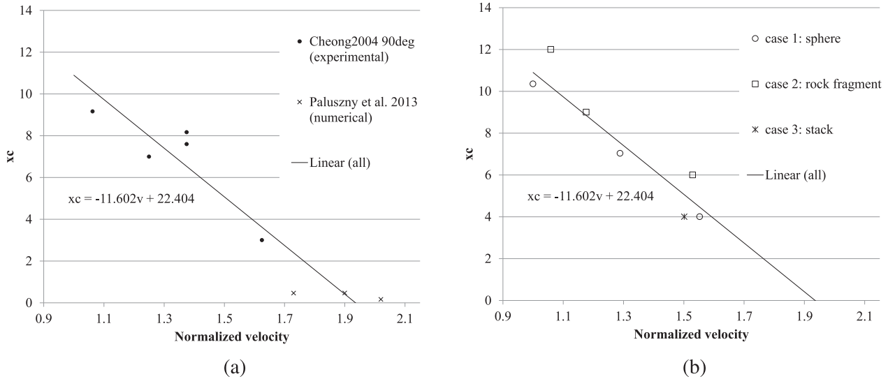
Fig. 7. Experimental relation between impact velocity and parameter x_c of the Weibull distribution: (a) experimental and numerical values, and (b) predicted values using the present method.
