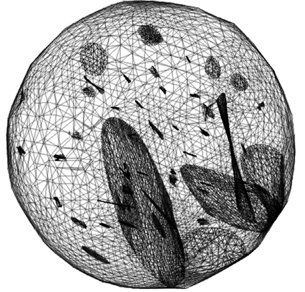
Fig. 5. FEM/DEM modeling of fracture-driven fragmentation (Paluszny et al., 2013). Fractures are propagated within each fragment using a velocity-dependent Paris propagation law which controls the relative velocity of fractures. These simulations generate fragment size distributions which conform with the expected Weibull distribution.
