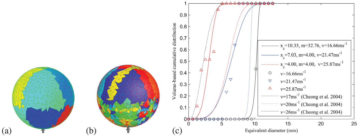
Fig. 9. Shape of fragments from the direct fragmentation of a single sphere with impact velocities (a) 17 m/s and (b) 26 m/s. Fragments are colored arbitrarily to distinguish them from each other. (c) Volume cumulative size distribution resulting from the fragmentation fitted by a two-parameter Weibull distribution equation.
