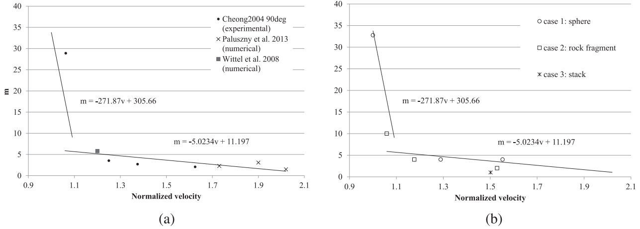
Fig. 6. Experimental relation between impact velocity and parameter m of the Weibull distribution: (a) experimental and numerical values, and (b) predicted values using the present method.
