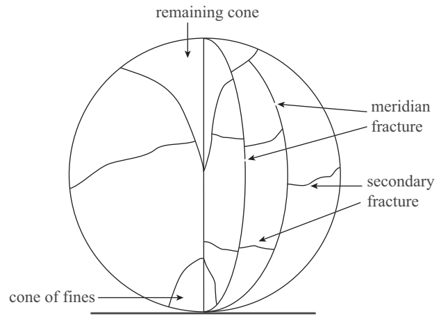
Fig. 1. Fragmentation pattern (adapted from Tomas et al., 1999).
